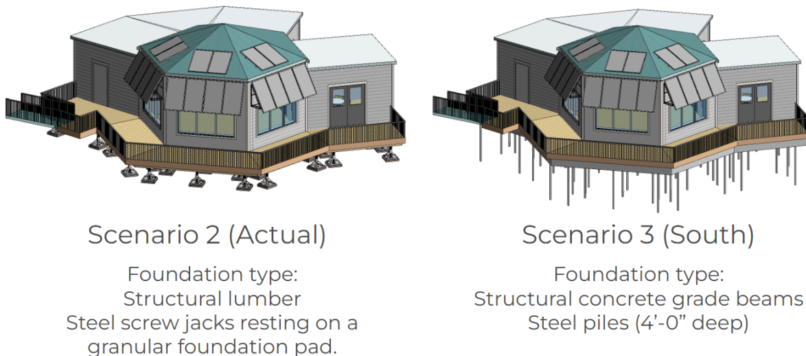
Figure 9: Scenario 2 and 3 foundation type comparison
